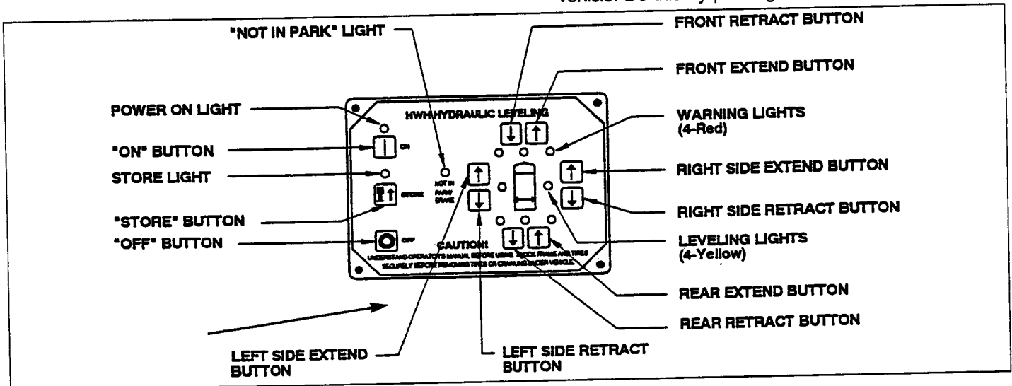
HYDRAULIC LEVELER PANEL
