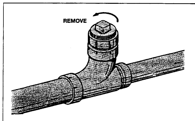
DRAIN CLEANOUT
